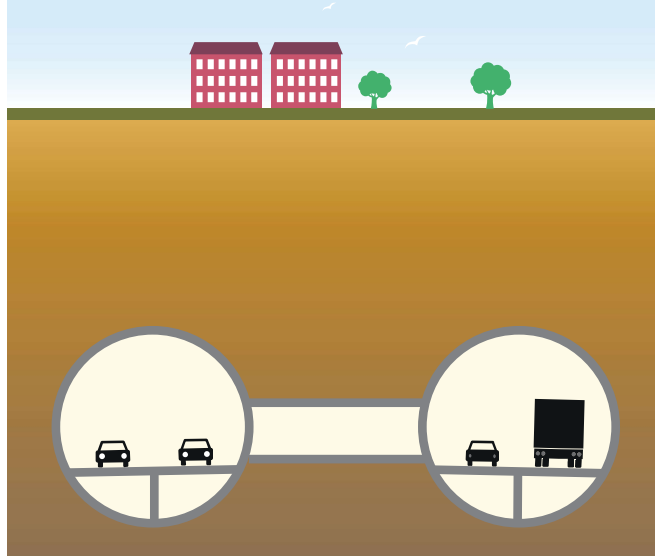
Figur 10: Boret tunnel.
