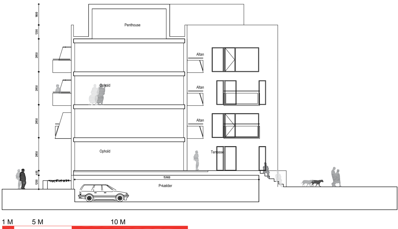
Snit A - A. Illustration: Catalyst Architects I/S.
