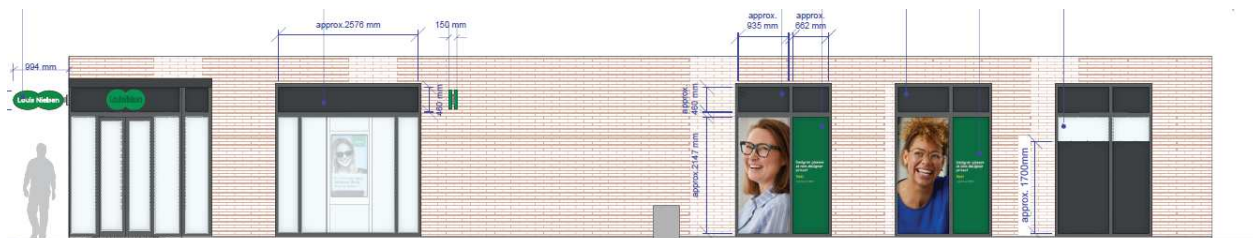
NORTH ELEVATION Scale 1:75
