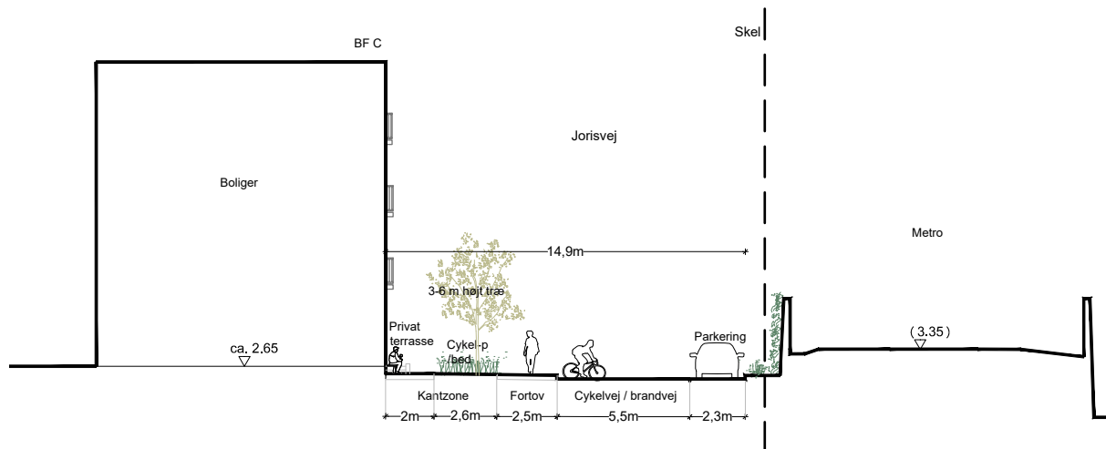
Snit A
