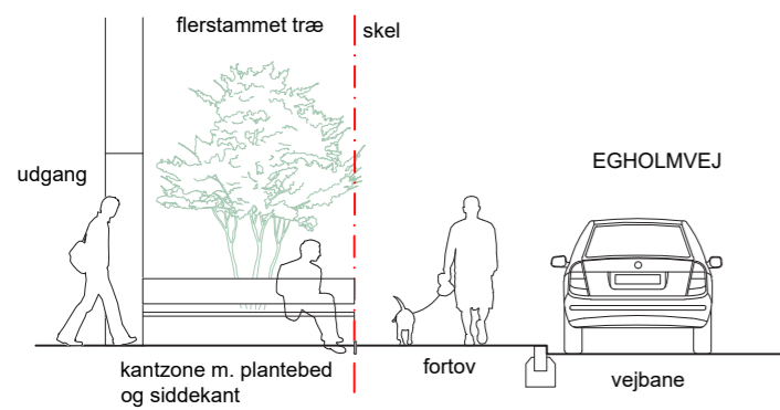
snit B
