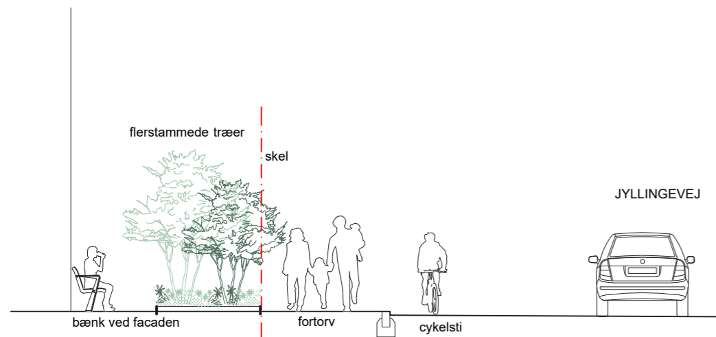
snit C
