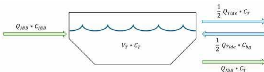
Figur 4-1 - Massebalance for stofkoncentration i Tømmergraven
