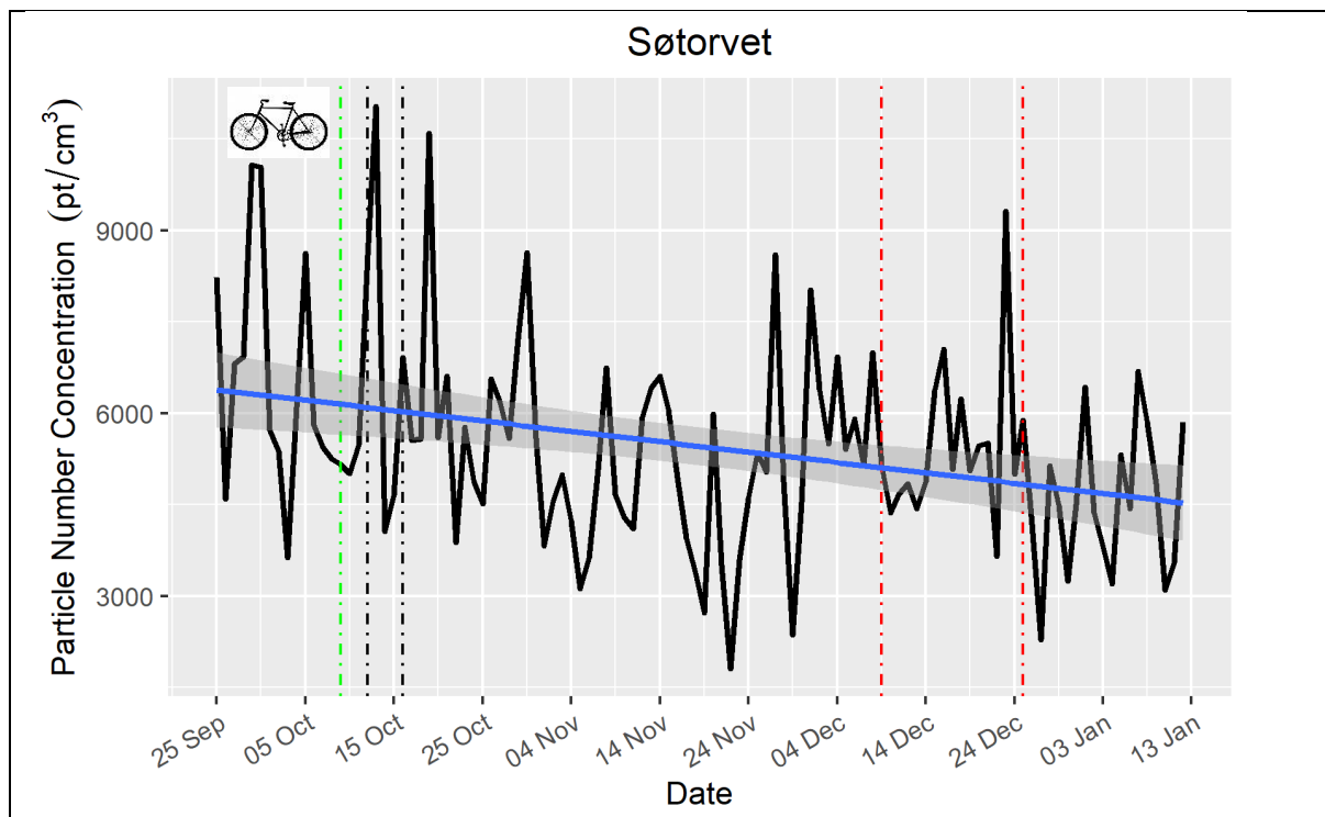
Figure 2. Daily mean PNC measured at S  torvet and Kr  gersgade UFP monitors between September 25 th , 2020, and January 15 th , 2021. Blue trendlines were added by applying linear models.
