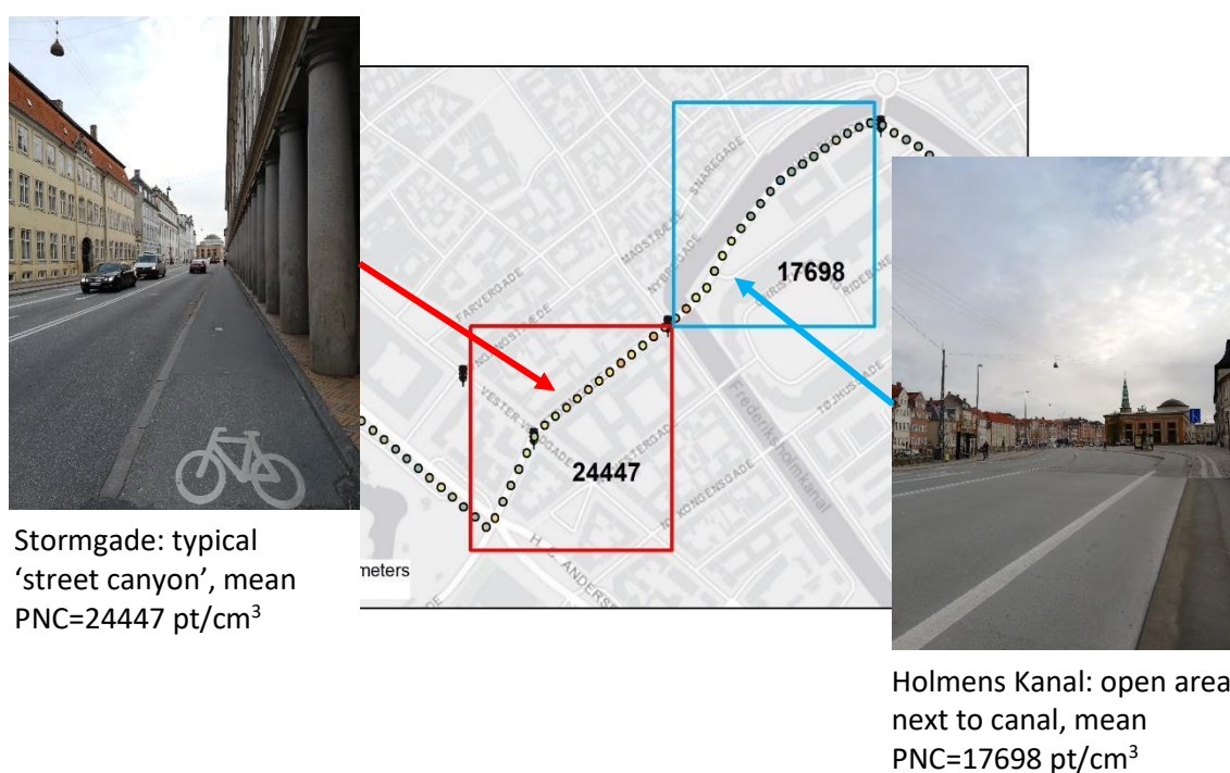
Figure 12. Mean PNC levels at Stormgade and Holmens Kanal (morning rush-hour, morning late, and afternoon rush-hour combined) on 28 weekdays during the study period (1st September until 9th of October, 2020).
