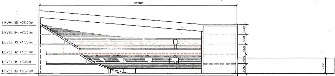
Example of an arena venue seating cross section
