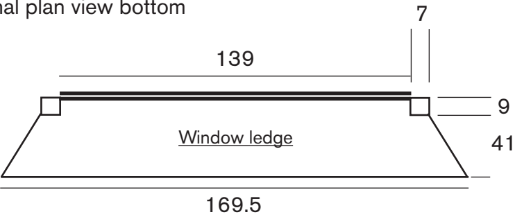
Internal plan view bottom
