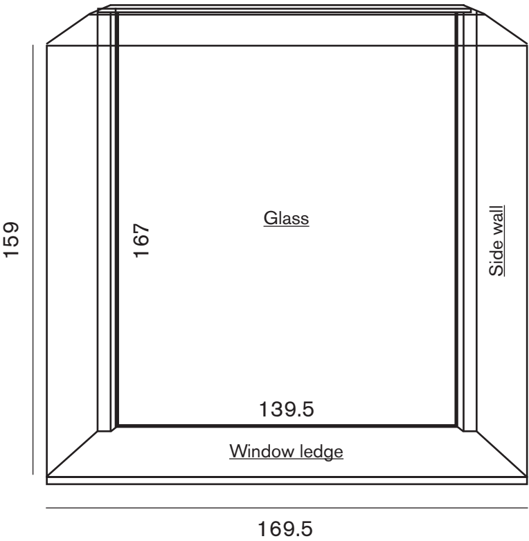
Internal plan view bottom
