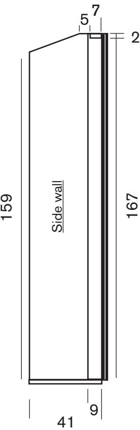
Internal view of side wall
