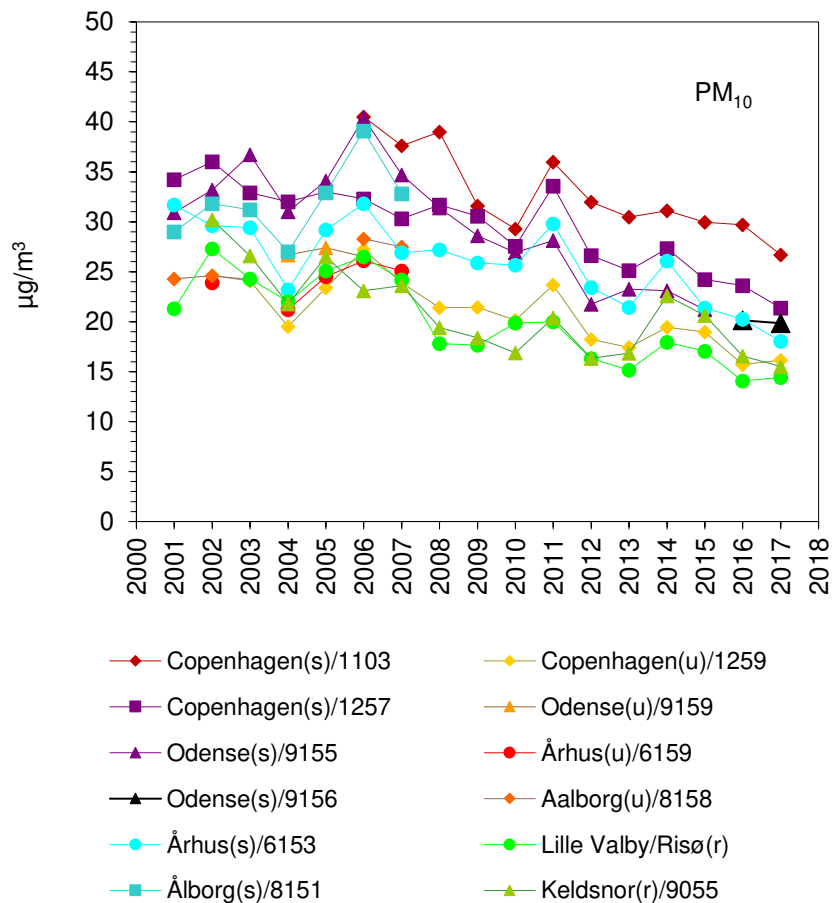
Figure 7.2. Annual averages for PM 10 measured at street stations (s), urban background stations (u) and at rural background stations (r). The change from gravimetric determination using the SM200 as a filter sampler to the use of the same instrument as a \beta -gauge from 2006 gives rise to a 5-10% increase due to the shift in method. Data are given at standard temperature- and pressure conditions (0°C and 1 atm.). PM given at ambient temperature and pressure conditions is on an annual average approximately 3-4% lower than PM-results given at standard conditions.
