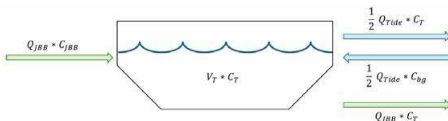
Figur 4-1 - Massebalance for stofkoncentration i Tømmergraven
