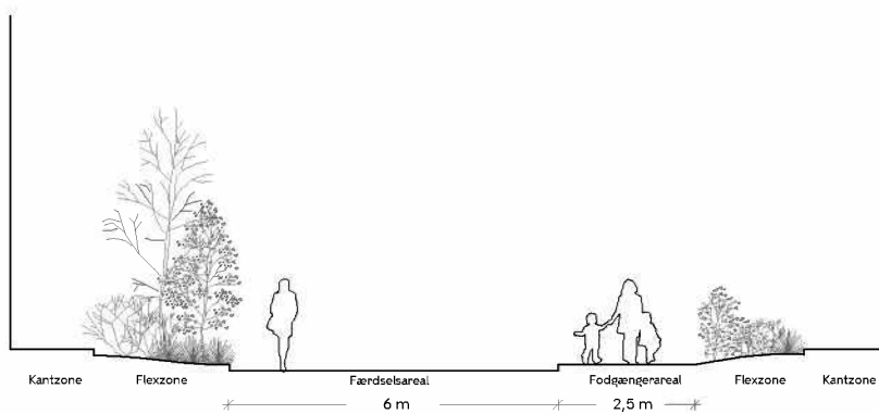
Snit C2
