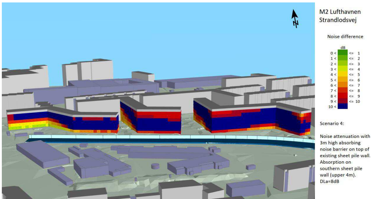
Figure 21 – Scenario 4. Noise reduction at residential façades with a 3 m high vertical absorptive barrier on the northern sheet-pile wall and absorptive elements installed on the upper 4 m of the southern sheet-pile wall.
