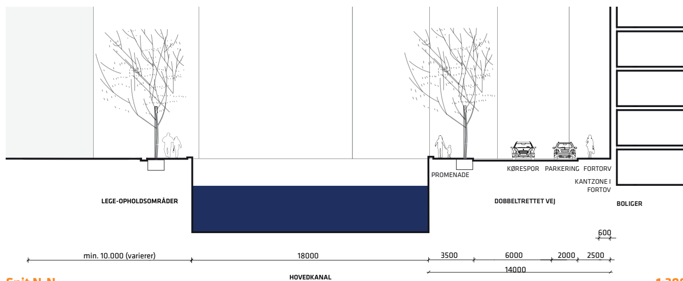
Snit N-N
