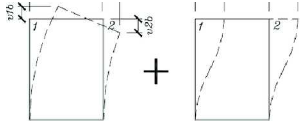
Bending Deformation
