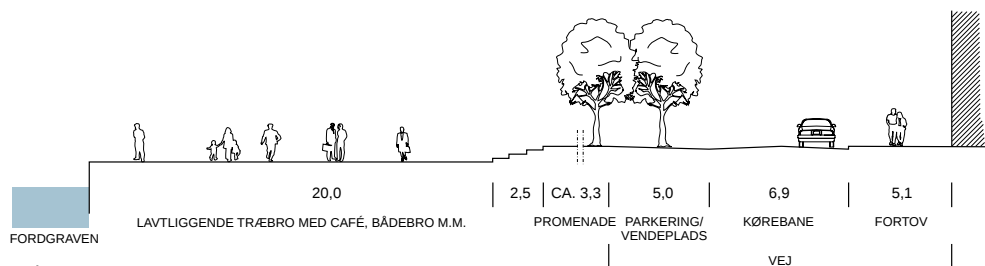
Snit H-H
