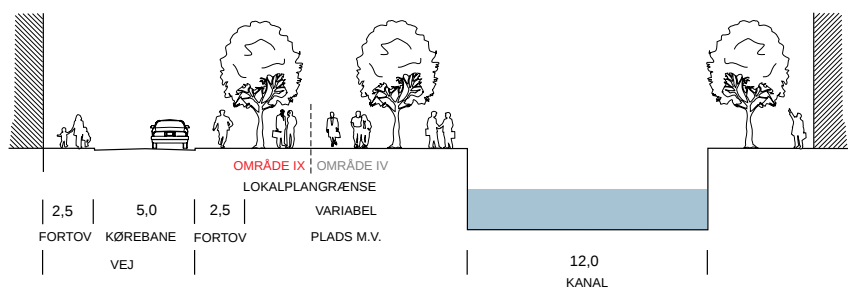
Snit F-F
