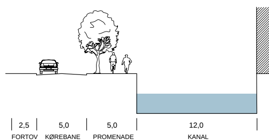
Snit K-K
