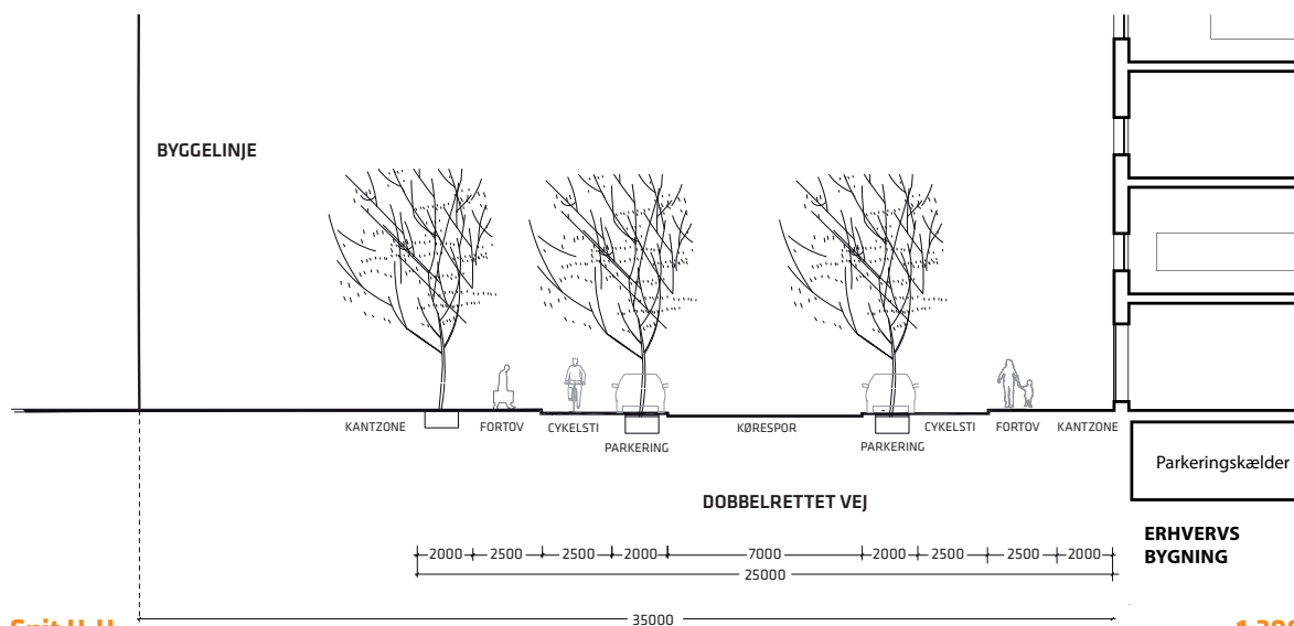
Snit H-H
