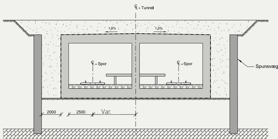
Figur 7.7 Cut og cover-tunnel under Mozarts Plads.
