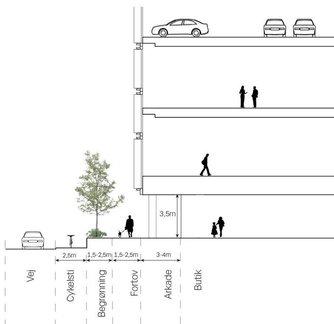
Snit J-J
