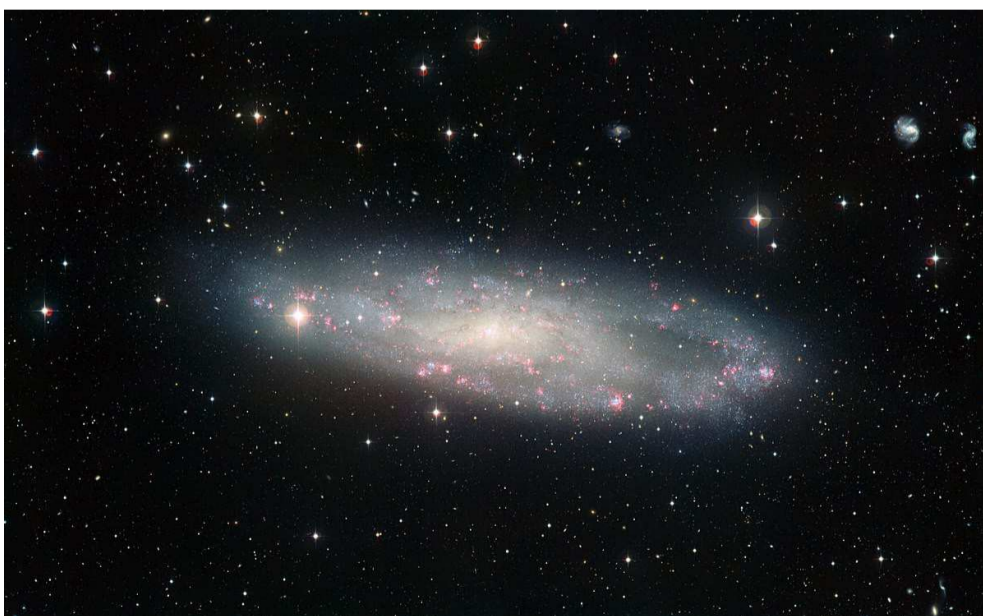
The NGC 247 spiral galaxy in the constellation Cetus (the Whale), photographed by La Silla Observatory, Atacama, Chile, 2011
