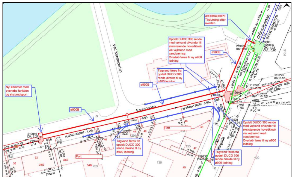
Figur 11 Principskitse for frakobling for Esplanaden.
