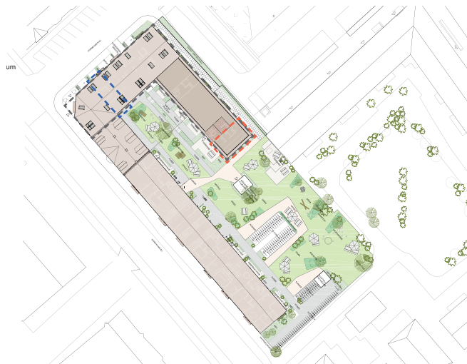
Situationsplan
