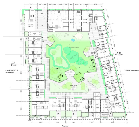
Situationsplan
