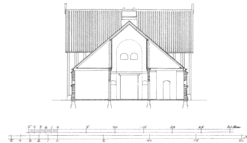
Snit
